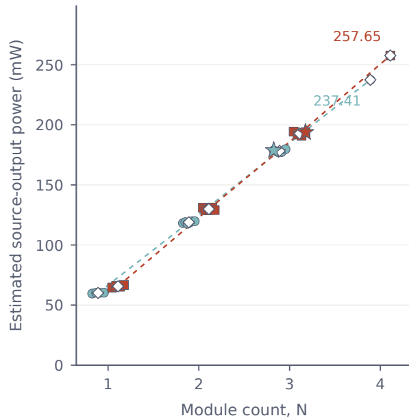
(b) Output power
